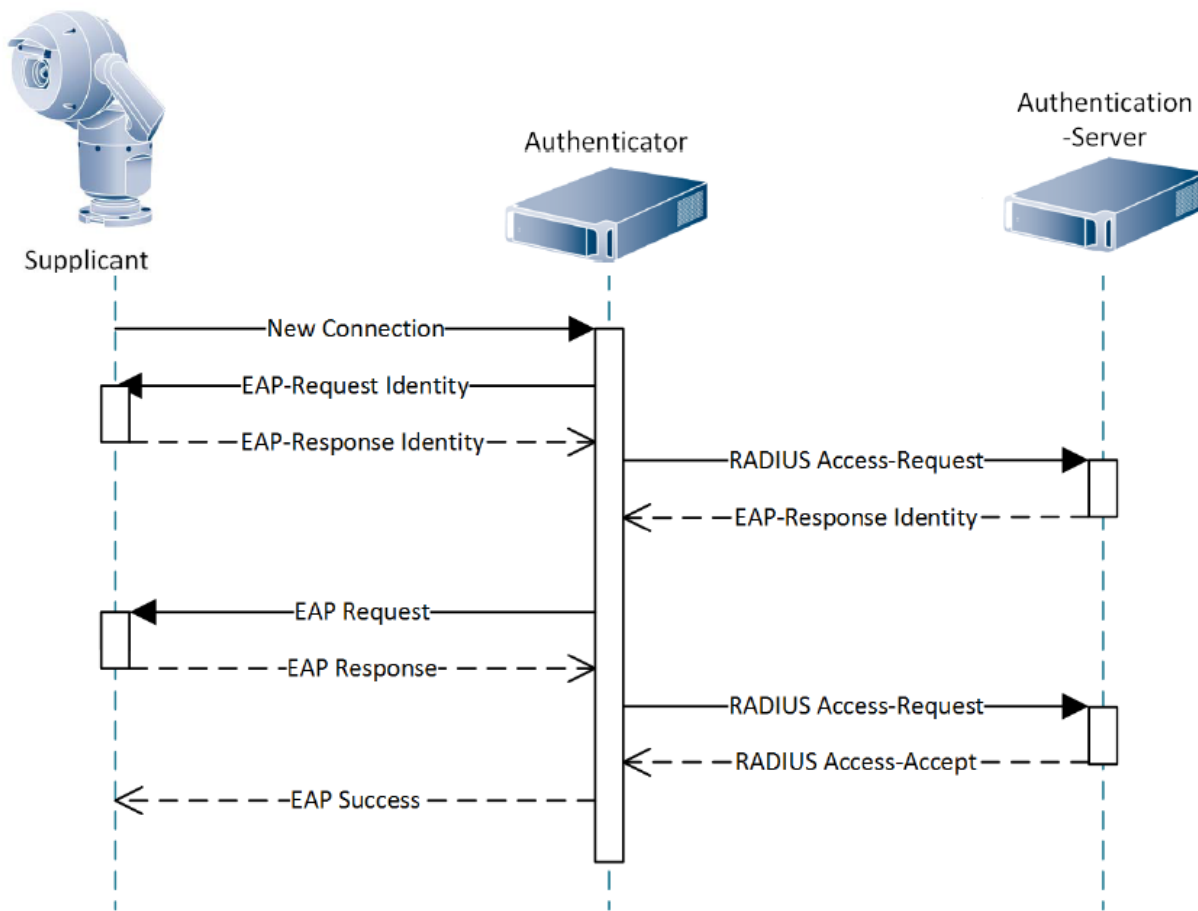
Figure - 802.1X Authentication Sequence Diagram
